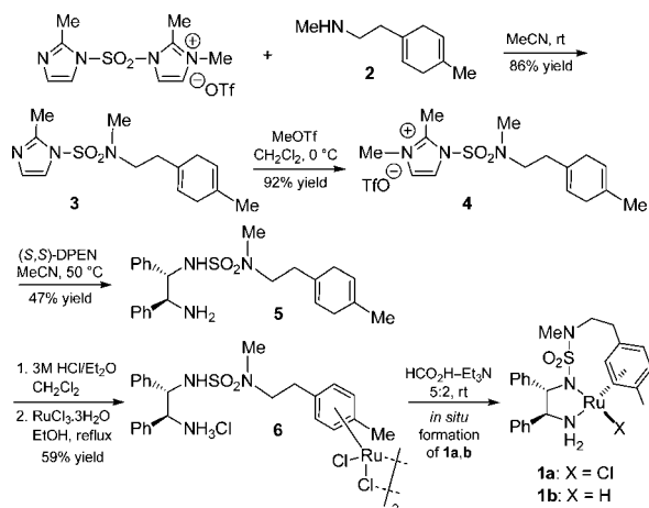
Scheme 1. Synthesis of the Active ansa -Type Ru(II) Complex 1b
