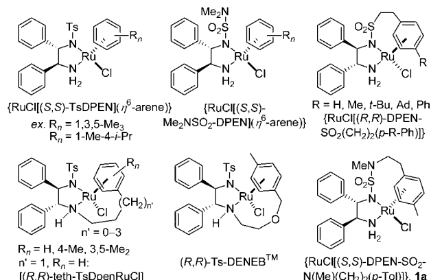
Figure 1. ATH Ru(II)-based precatalysts.
